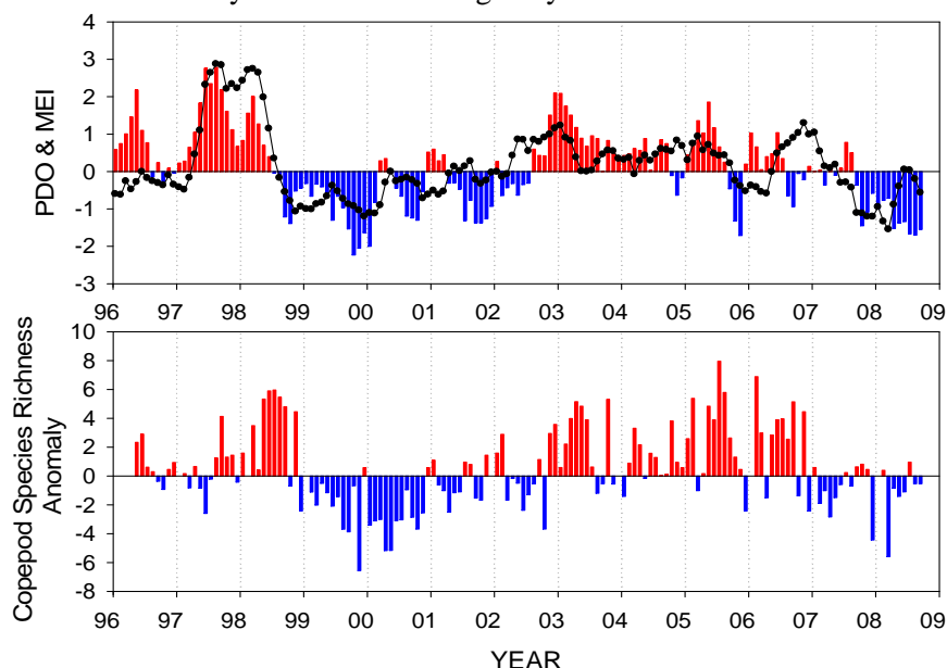
Figure 9. Time series of the monthly values of PDO, MEI and copepod species richness. Note that species richness tracks the PDO and MEI fairly closely; also note that richness has had negative anomalies since 2007.
