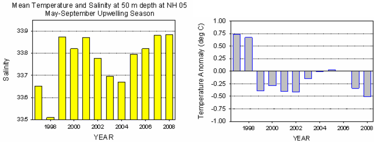
Figure 7. Salinity in deep water at station NH 05, 1997-present, averaged from May-September (Left). Temperature anomalies for the same period (Right). Note that the summer of 2008 was colder and saltier than other years.
