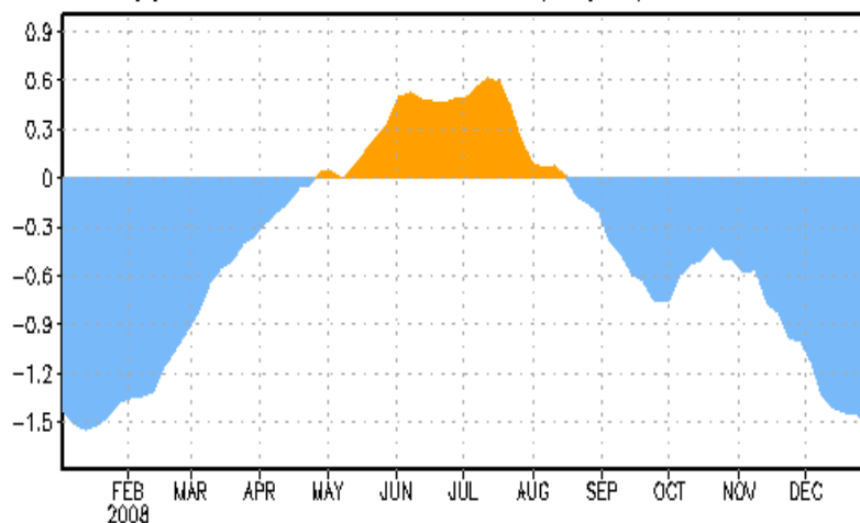
Figure 2. Area-averaged upper-ocean heat content anomalies (°C) in the equatorial Pacific (5°N-5°S, 180°-100°W). Heat content anomalies are computed as departures from the 1982-2004 base period pentad means. The upper ocean heat content was below-average across the eastern half of the equatorial Pacific Ocean between January 2007 and April 2008, and above-average from early May 2008 through mid-August 2008. Since mid-August 2008, the heat content anomalies have been below-average. The negative heat content anomalies have strengthened since mid-October 2008.
