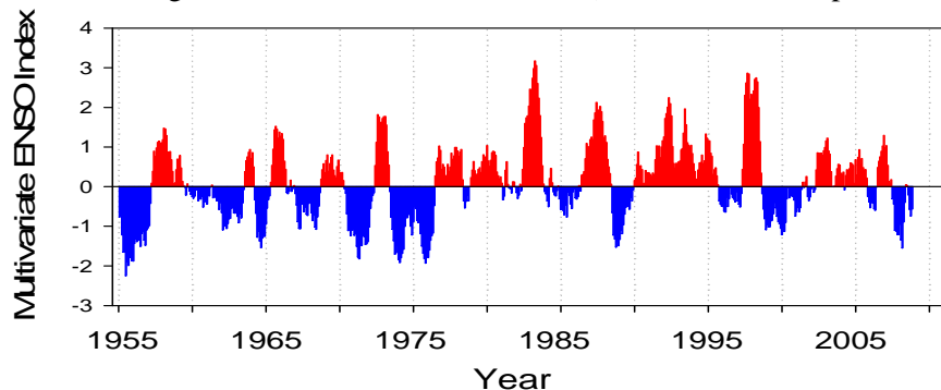
Figure 1. Time-series of the Multivariate ENSO Index (MEI), 1955 to 2008. Note the extended period of weak El Niño conditions (positive values) from 2002-2006 and the La Niña conditions (negative values) since 2007.
