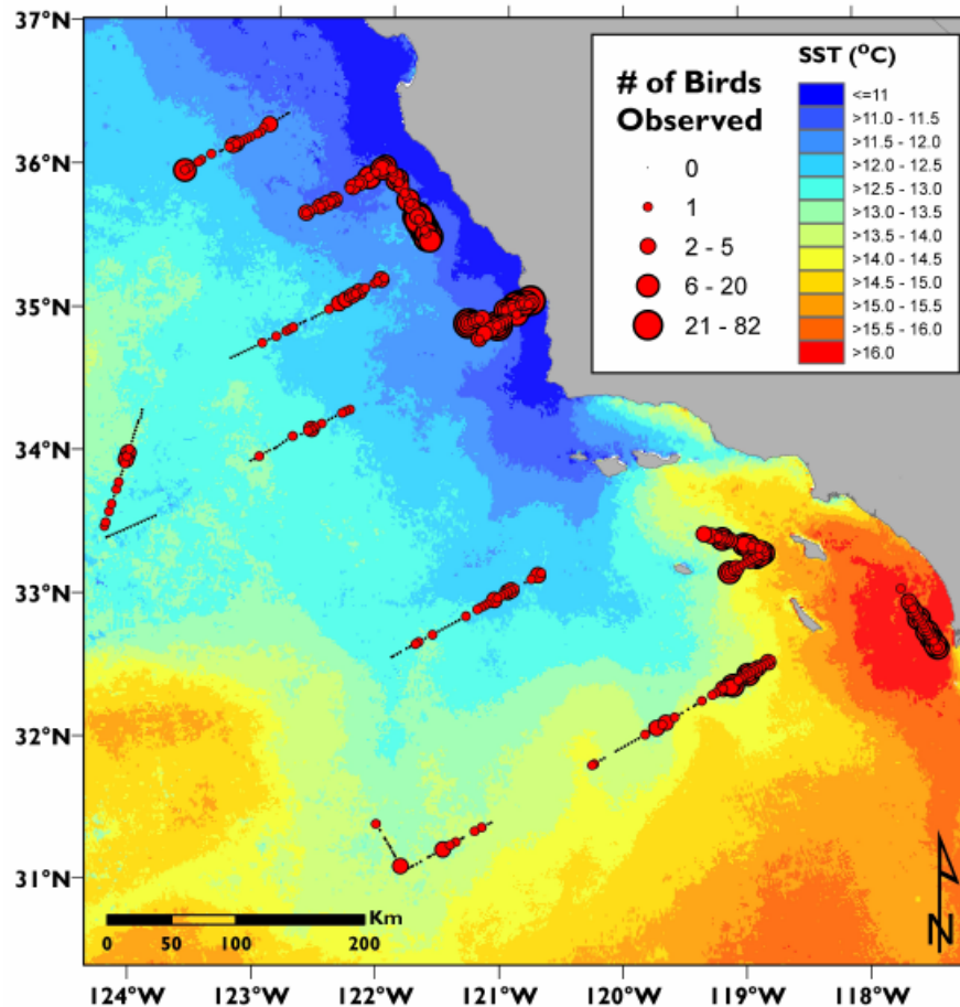
Figure 18. Along-transect spatial pattern of all birds counted in April 2008 overlaid on a monthly composite of satellite sea surface temperature.
