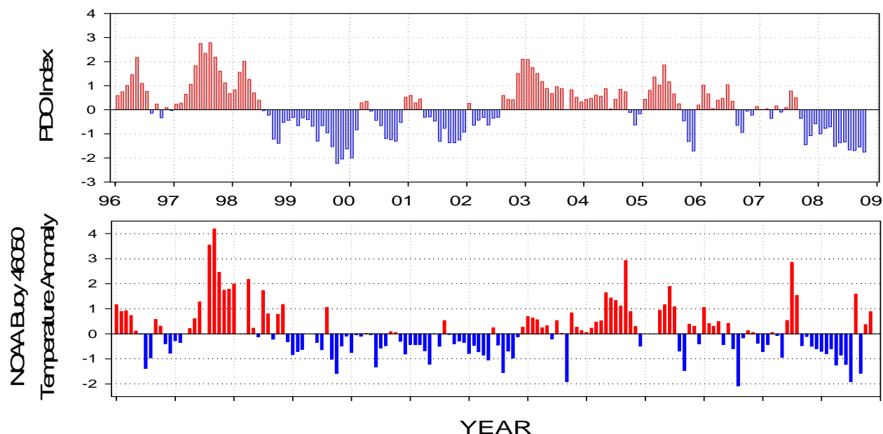
Figure 6. Time series of monthly PDO (upper) and the monthly temperature anomalies at the NOAA Buoy 46050 (lower) since 1996. Note the close association of the PDO with SST.
