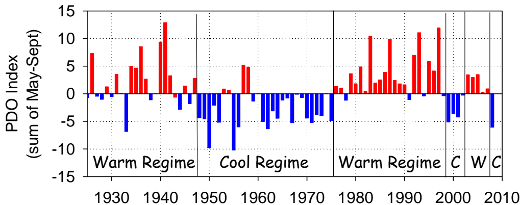
Figure 3. Time series of the PDO summed over May-September, 1925 to 2008. Note that the summer-time value in 2008 was the most negative since 1956.
