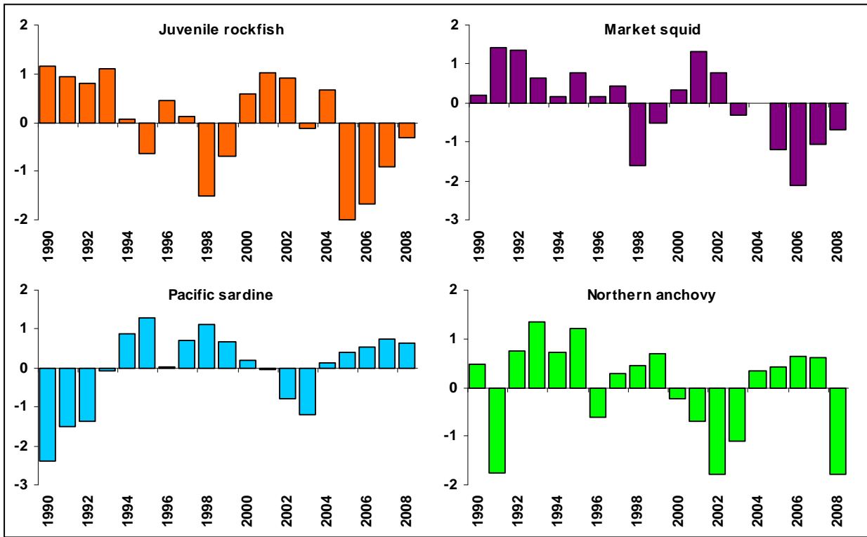
Figure 11. These graphs show the standardized anomalies from the log of mean values by year for four key forage species that are well sampled in this survey. There is typically strong covariance among the ten most frequently encountered rockfish species in the survey. However in 2008 most of the rockfish observed were “northern” species such as widow, canary, and yellowtail rockfish, while the traditionally most abundant species in this region, particularly shortbelly rockfish, remained at record low levels. Market squid were also encountered at below average numbers in 2008, but had increased over the 2005-2007 period. By contrast, Pacific sardine numbers were down modestly in 2008, and northern anchovy numbers were down significantly, relative to the 2005-2007 period.
