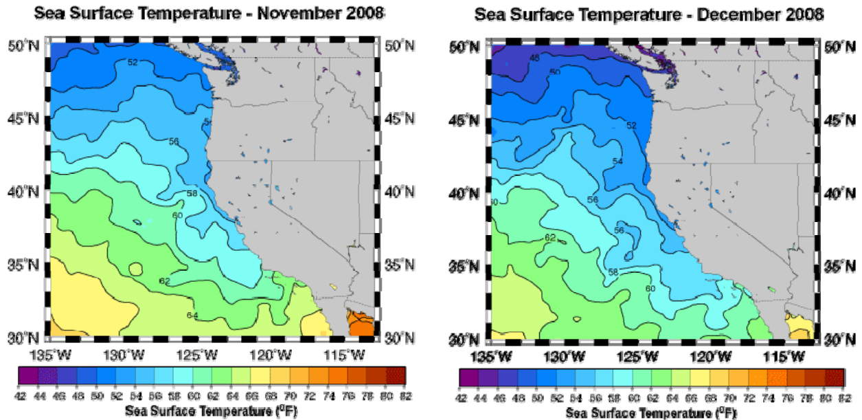
Figure 5. Regional oceanic conditions along the California current.
