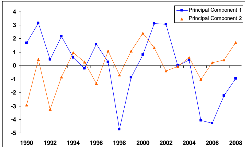
Figure 12. The first and second principle components.
