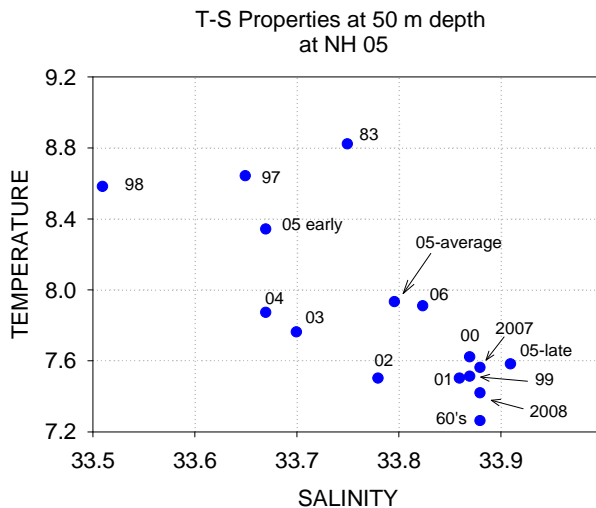
Figure 8. A plot of temperature and salinity, using values averaged over May-September from deep water at station NH-05. Note that 2008 is the coldest of the time series which began in 1997, but not as cold as the deep water temperatures averaged for data from the 1960s.
