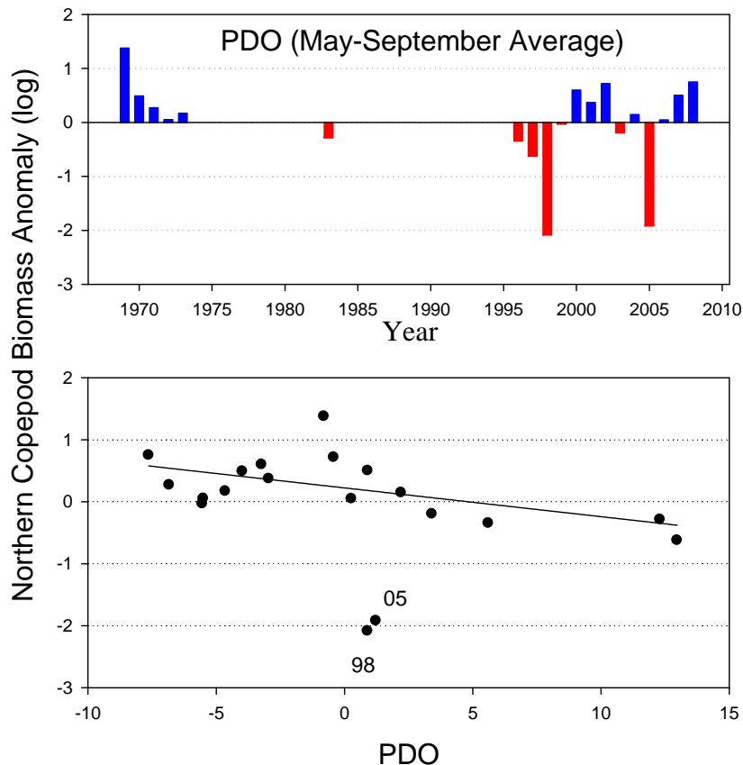
Figure 10. Northern copepod biomass anomalies from station NH-05, Oregon, including historical data (1969-1973, 1983) and data from 1996-present. The value of the biomass anomaly for 2008 is similar to values seen in 2000 and 2002.
