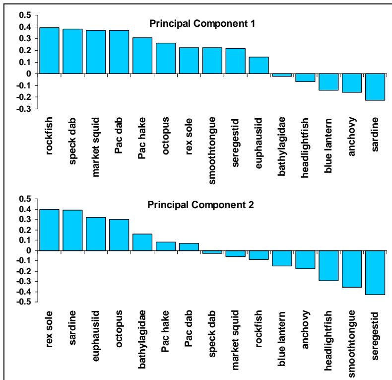
Figure 13. The loadings of the first and second principle components.
