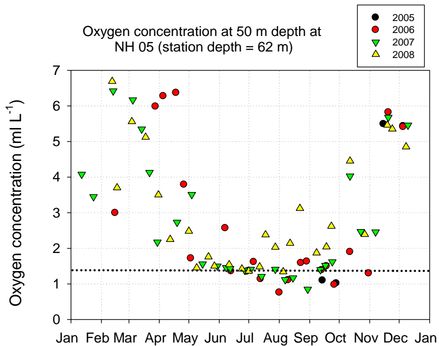
Figure 20. Oxygen concentration at station NH 05 (five miles off Newport, Oregon, along the Newport Hydrographic Line), at a depth of 50 m. Note that during 2008 (yellow triangles), oxygen concentrations were higher during summer months as compared to the past two years. Hypoxic conditions (oxygen concentrations less than 1.4 ml per Liter) were only observed in early August.
