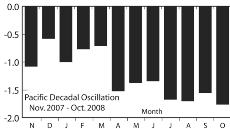
Figure 4. This graph presents monthly values for the PDO Index from November 2007 to October 2008 ( http://jisao.washington.edu/pdo/ ). The October PDO index is the most extreme of the current series of negative values. The last four monthly PDO indices were the first since January 2000 to have values less than or equal to -1.55.
