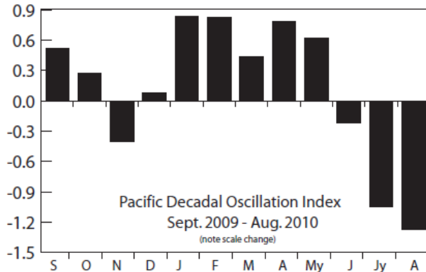
Figure 3. Monthly values for the PDO Index for September 2009 through August 2010. September PDO index value was -1.61.
